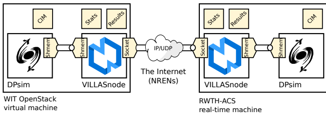
Fig. 2. Co-simulation architecture.
