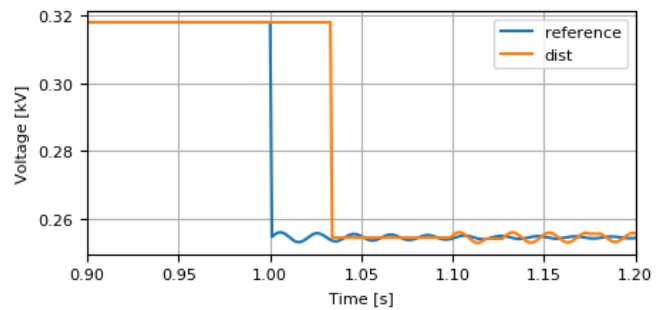
Fig. 10. Comparison of integrated reference simulation and distributed co-simulation among RWTH and WIT.
